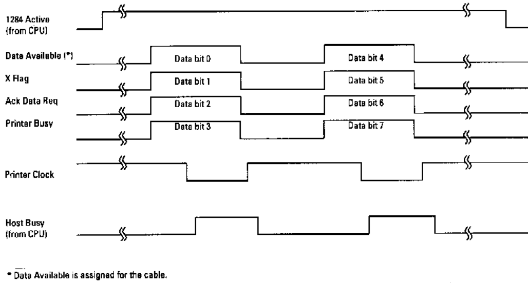
Figure C-2 Data transmission timing
